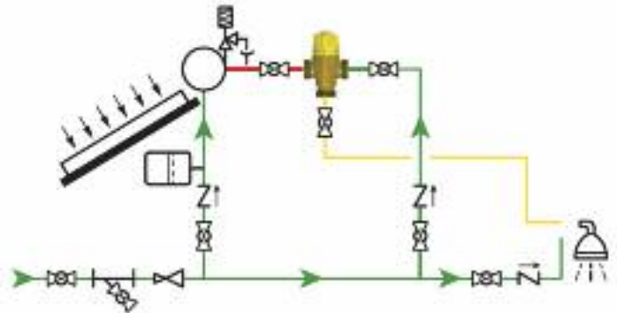
Natural circulation solar system
